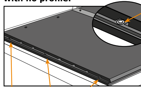
fasten edge of upper mat with 3 fastening elements
